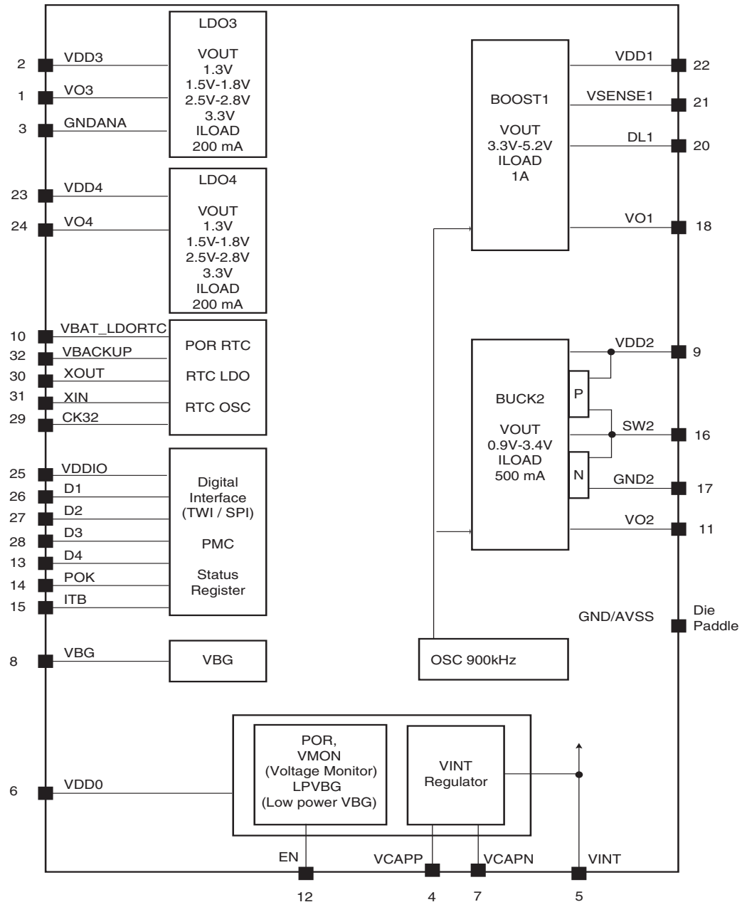
Figure 2-1. Block Diagram
