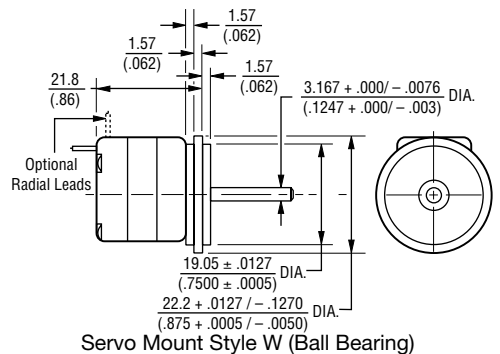
Servo Mount Style W (Ball Bearing)
