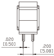
M7 Double Pole
