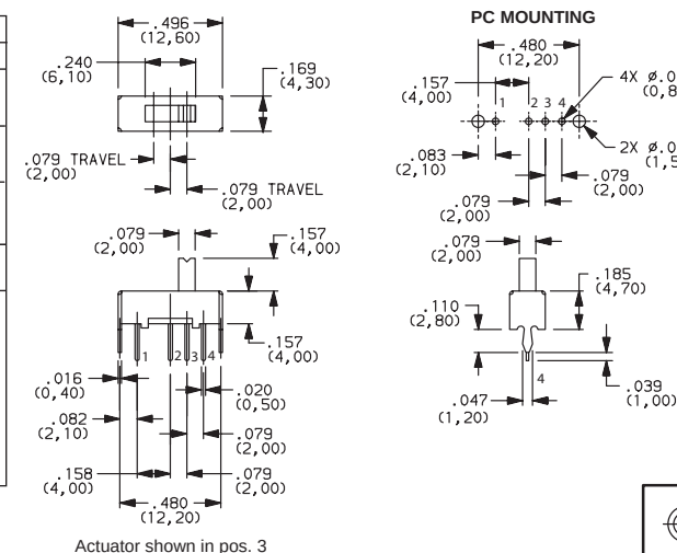
OS103011MS8QP1 SP3T
