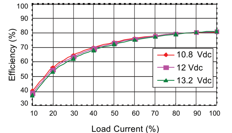
PCN2-S12-D5-S Efficiency Curve (Efficiency vs. Line Voltage and Load Current)
