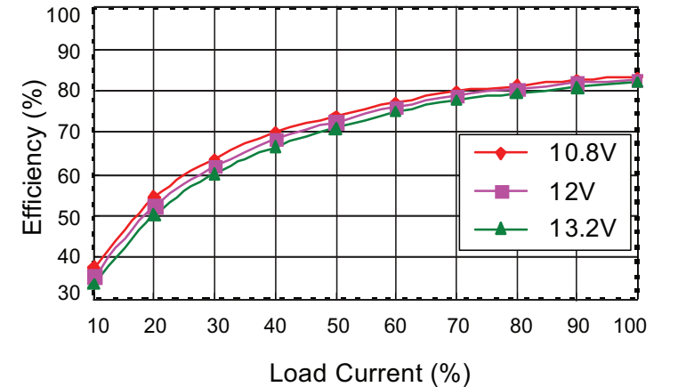
PCN2-S12-S12-S Efficiency Curve (Efficiency vs. Line Voltage and Load Current)
