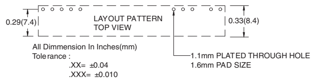
Figure 5. Recommended VPOL15A-5-SIP Footprint
