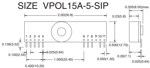
Figure 16 VPOL15A-5-SIP Mechanical Outline Diagram
