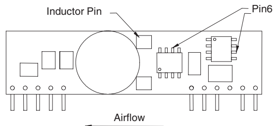
Figure 7. Temperature Measurement Location for VPOL15A-5-SIP
