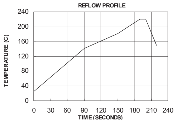
Figure 15 VPOL16A-12-SIP Reflow Profile
