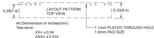
Figure 5. Recommended VPOL16A-12-SIP Footprint
