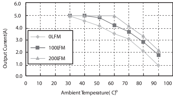
Figure 2. Typical Power De-rating for 12V IN 3.3Vout
