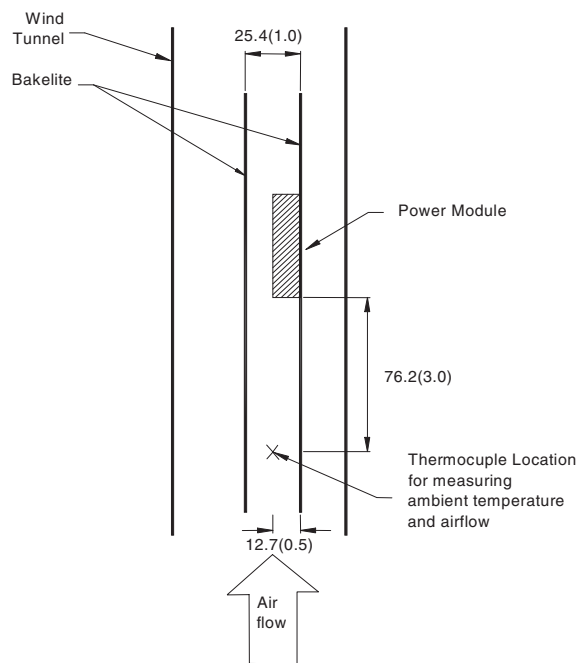
Figure 6. Thermal Test Setup
