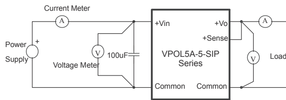
Figure 11. VPOL5A-5-SIP Series Test Setup
