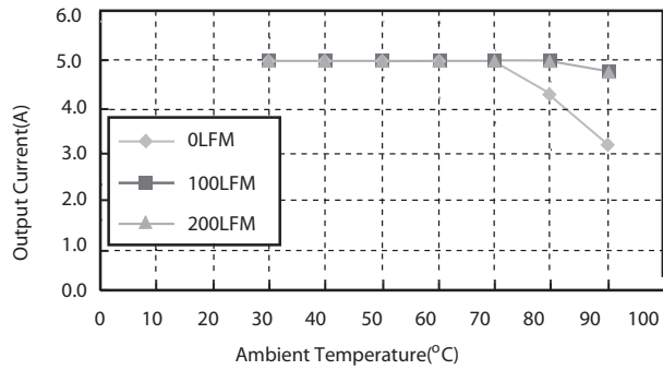
Figure 2. Typical Power De-rating for 5V IN 3.3Vout
