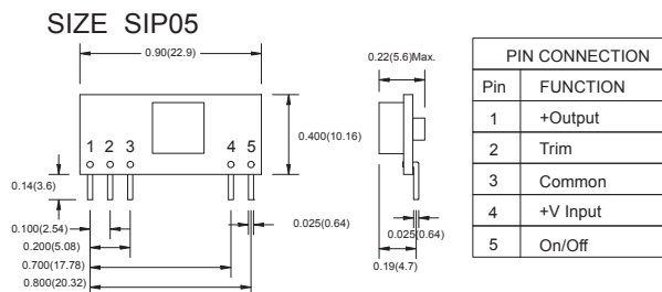
Figure 14 VPOL5A-5-SIP Mechanical Outline Diagram
