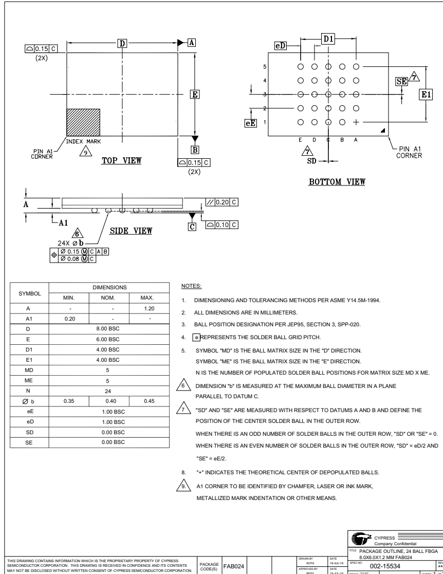
Figure 6.9 Ball Grid Array 24-Ball 6x8 mm (FAB024)
