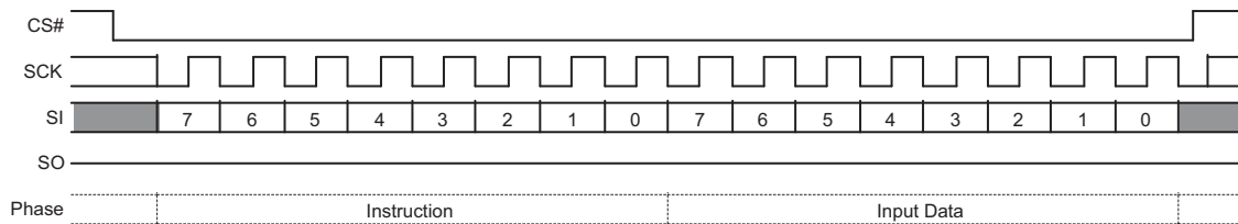
Figure 3.4 Single Bit Wide Input Command
