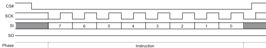
Figure 9.71 Deep Power-Down Command Sequence
