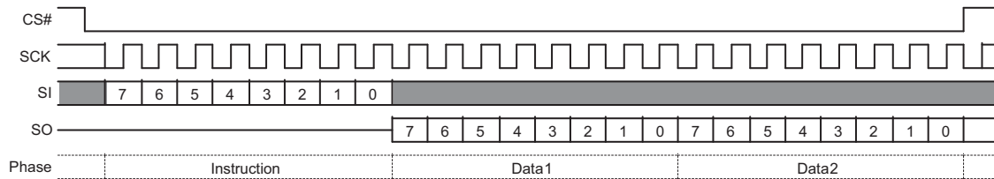
Figure 3.6 Single Bit Wide I/O Command without Latency
