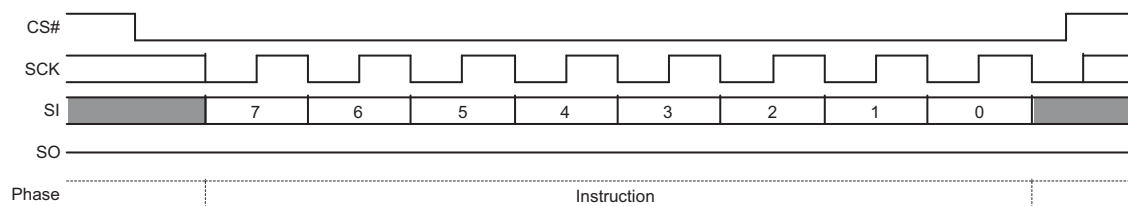
Figure 9.51 Erase or Program Resume Command Sequence
