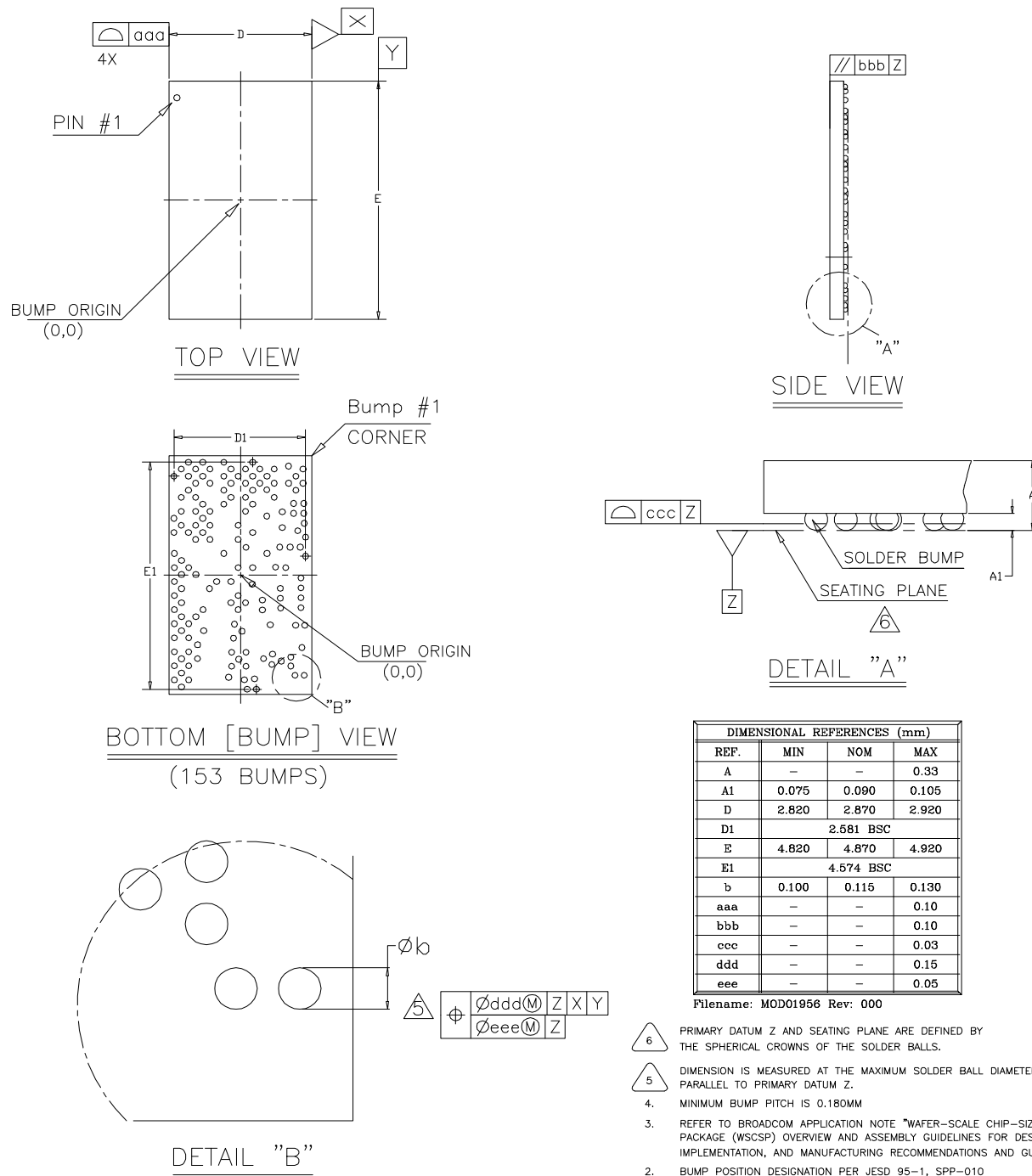
Figure 36. 153-Bump WLCSP Mechanical Information
