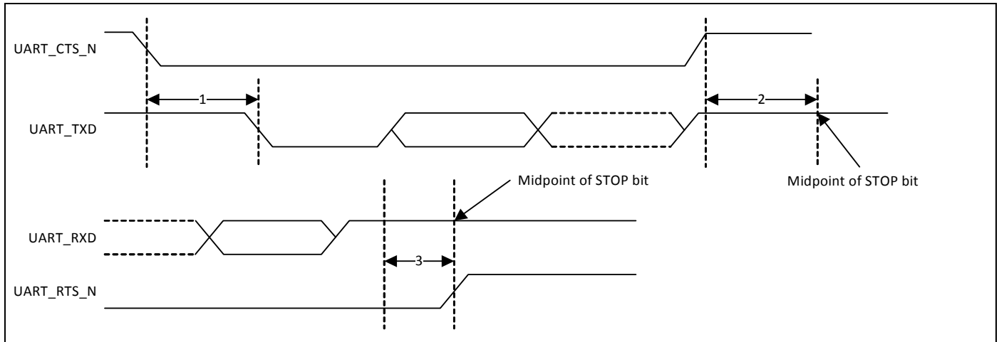
Figure 19. UART Timing
