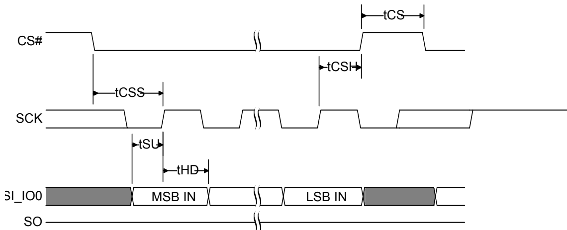
Figure 143. SPI Single Bit Input Timing
