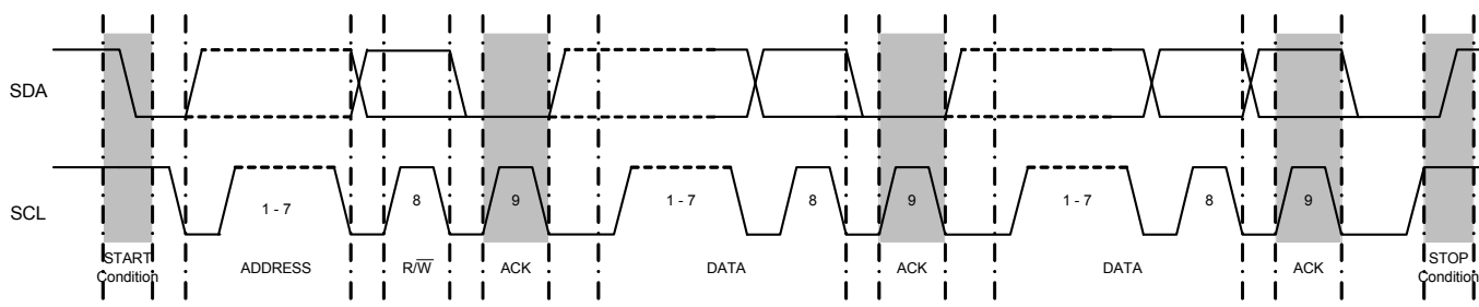
Figure 7-18. I²C Complete Transfer Timing
