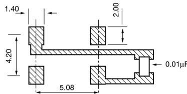
Figure 2) Land Pattern
