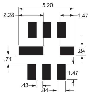
Figure 2) Land Pattern
