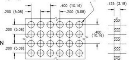
PANEL HOLE PATTERN 4 PIN / 6 PIN MODULE
