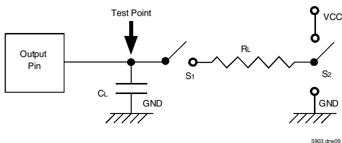
Figure 7. Output Load
