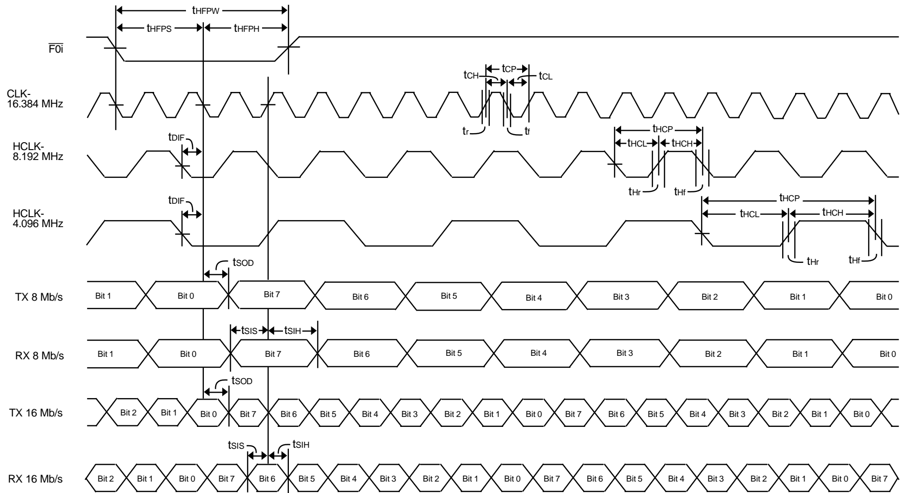
Figure 14. WFPS Timing
