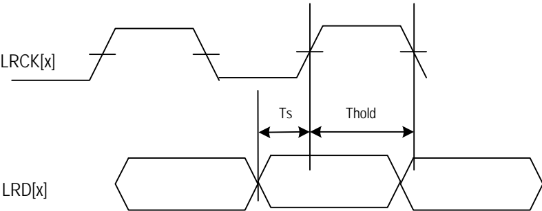
Figure 93. Receive Line Interface Timing
