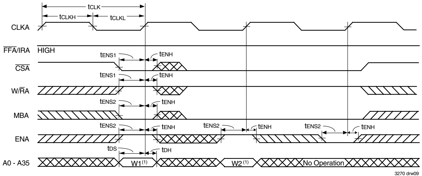
Figure 7. Port A Write Cycle Timing for FIFO1 (IDT Standard and FWFT Modes)
