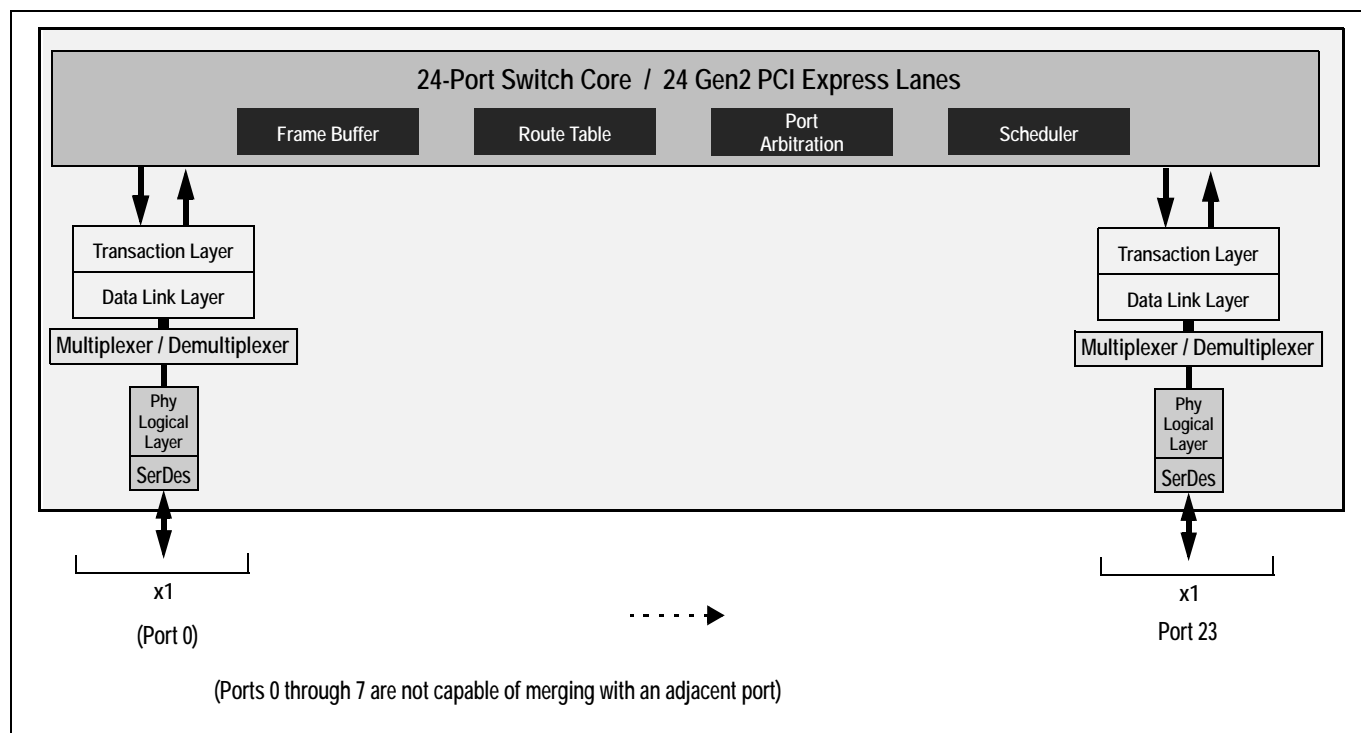
Figure 1 PES24NT24G2 Block Diagram
