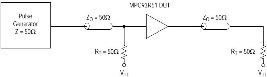
Figure 10. CLK MPC93R51 AC Test Reference for VCC = 3.3 V
