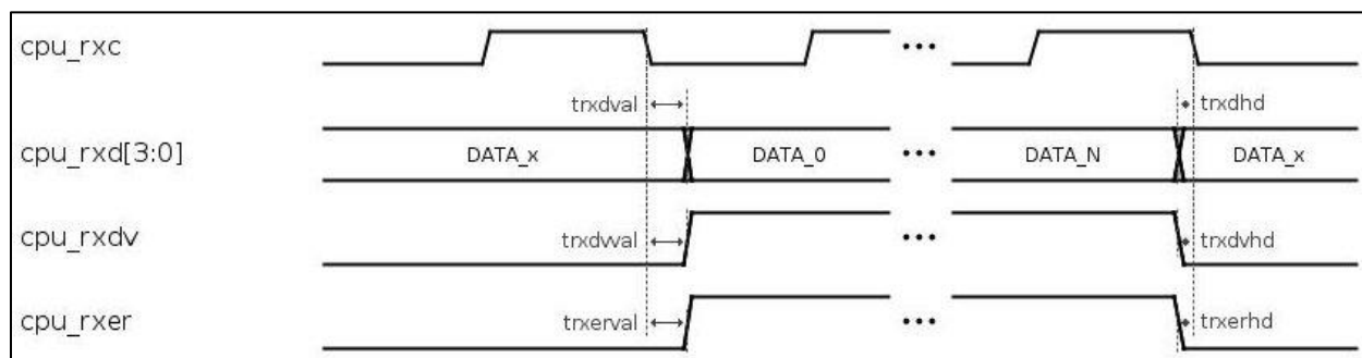
Figure 15 Internal MII Interface, TRANSMIT DATA
