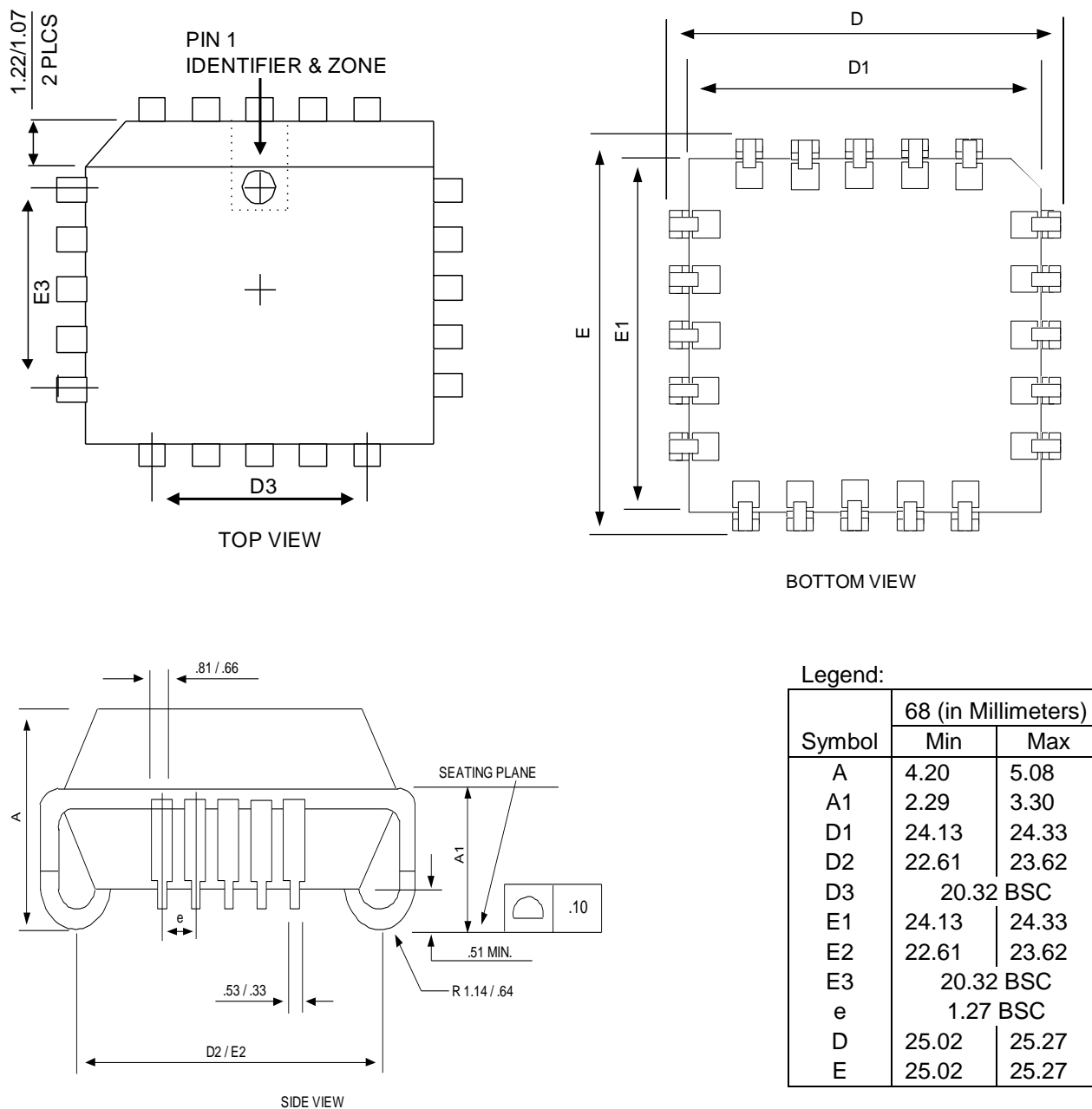
Figure 3. Package Dimensions
