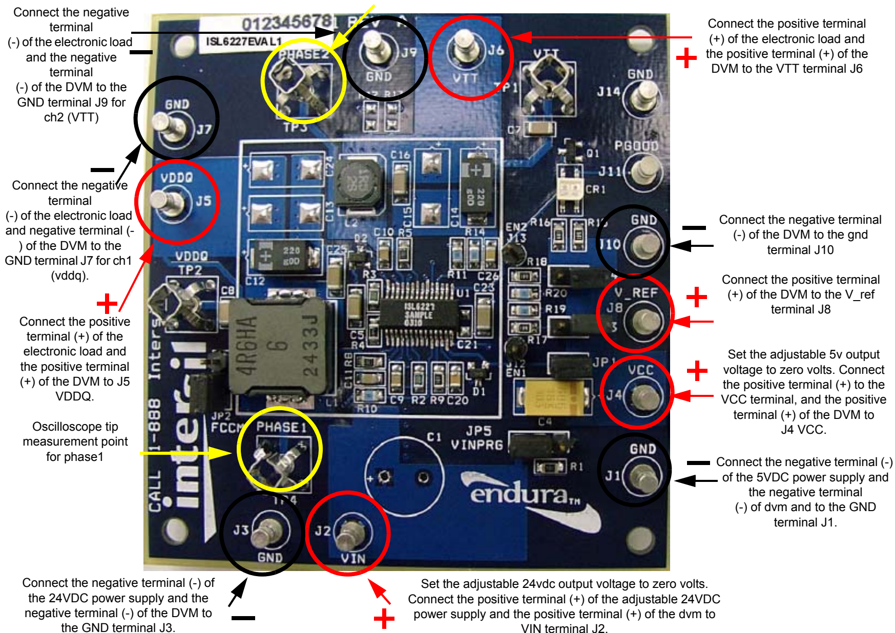
FIGURE 2. WIRING CONNECTIONS FOR ISL6227EVAL1 (see Quick Setup)
