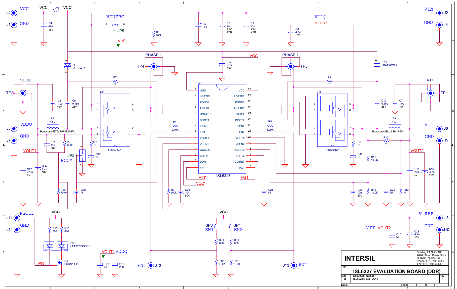
FIGURE 3. ISL6227EVAL1 SCHEMATIC
