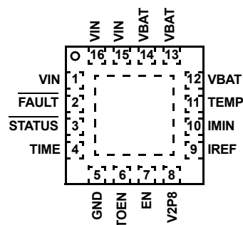
ISL6298 (16 LEAD QFN) TOP VIEW
