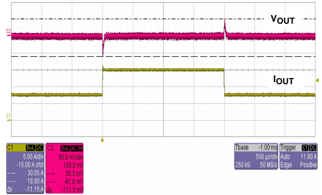
FIGURE 6. TRANSIENT RESPONSE
