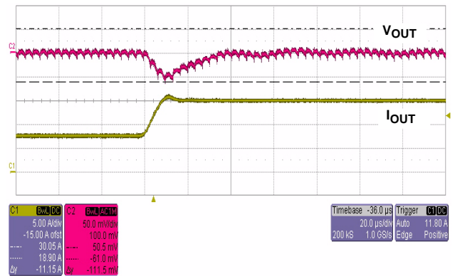
FIGURE 7. TRANSIENT RESPONSE
