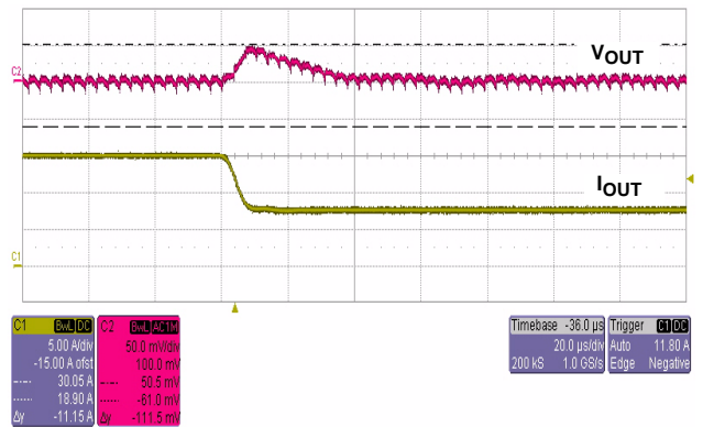
FIGURE 8. TRANSIENT RESPONSE
