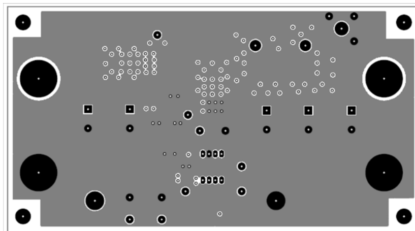
FIGURE 14. ISL8105AEVAL1Z - LAYER 2
