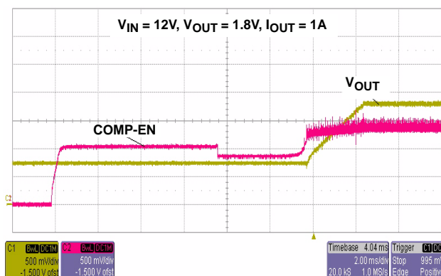
FIGURE 3. SOFT-START WITH PRE-BIASED OUTPUT
