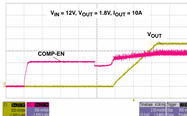
FIGURE 2. SOFT-START
