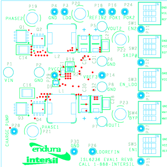
FIGURE 3. TOP COMPONENTS
