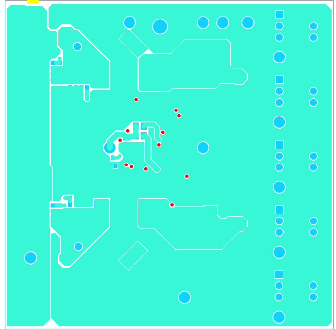
FIGURE 4. TOP ETCH
