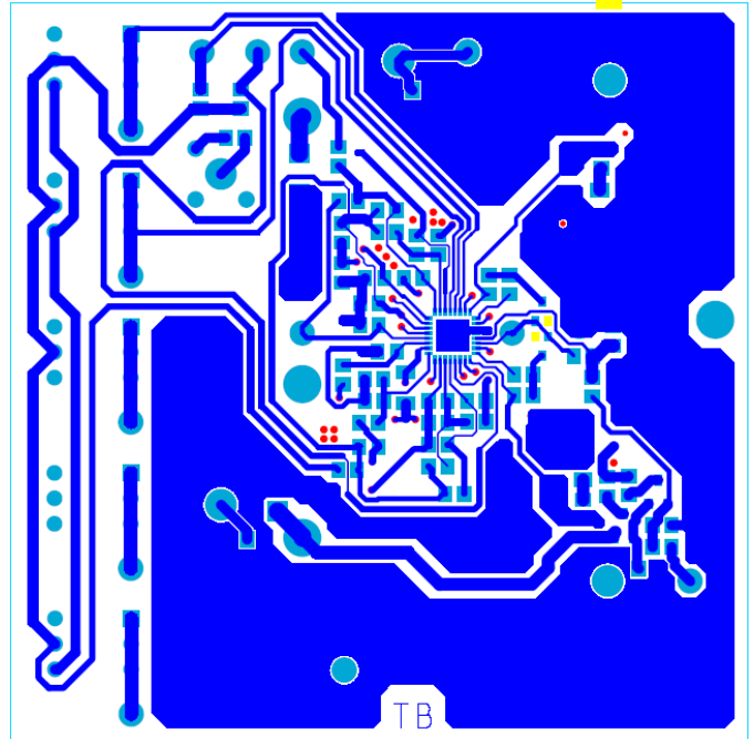
FIGURE 8. BOTTOM ETCH (MIRRORED)
