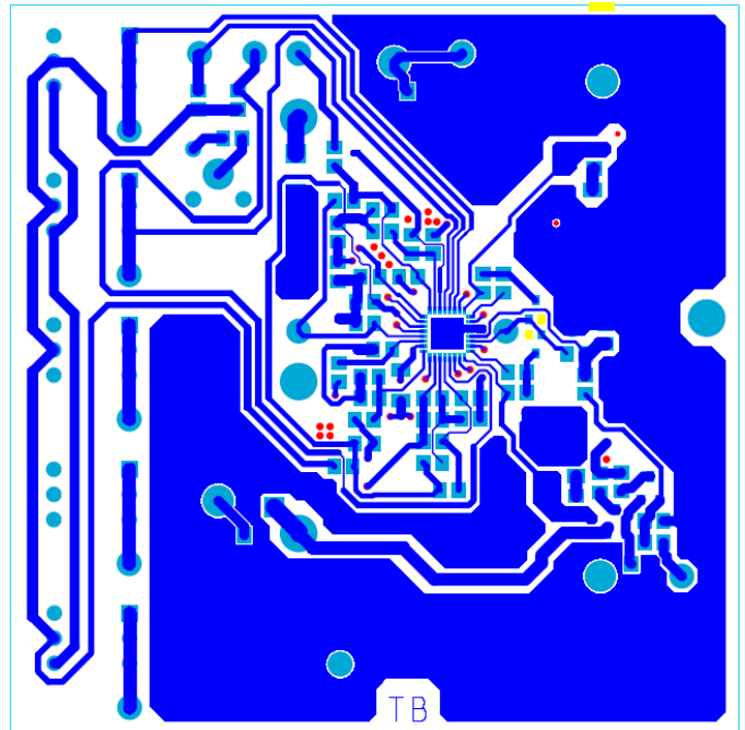
FIGURE 7. BOTTOM ETCH (MIRRORED)
