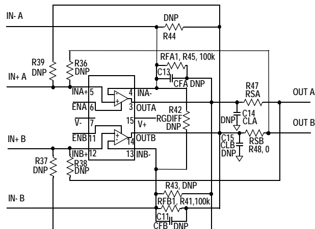
FIGURE 5. OPTIONAL COMPONENTS
