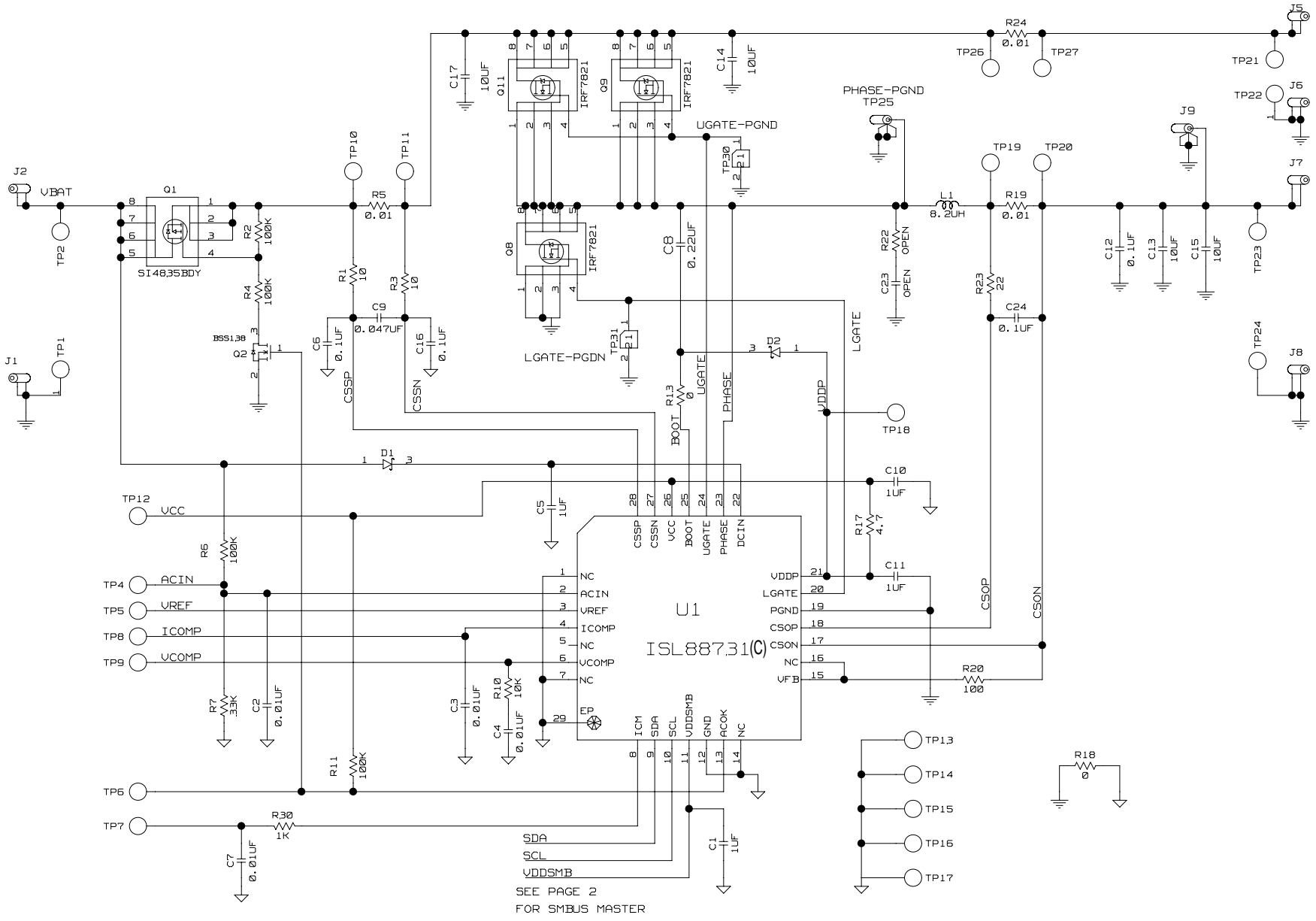
FIGURE 10. ISL88731(C)EVAL2Z SCHEMATIC
