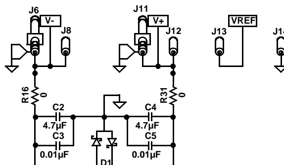
FIGURE 1. POWER SUPPLY CIRCUIT
