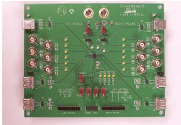
FIGURE 1. ISL540230EVAL2Z, ISL540230EVAL3Z EVALUATION BOARD
