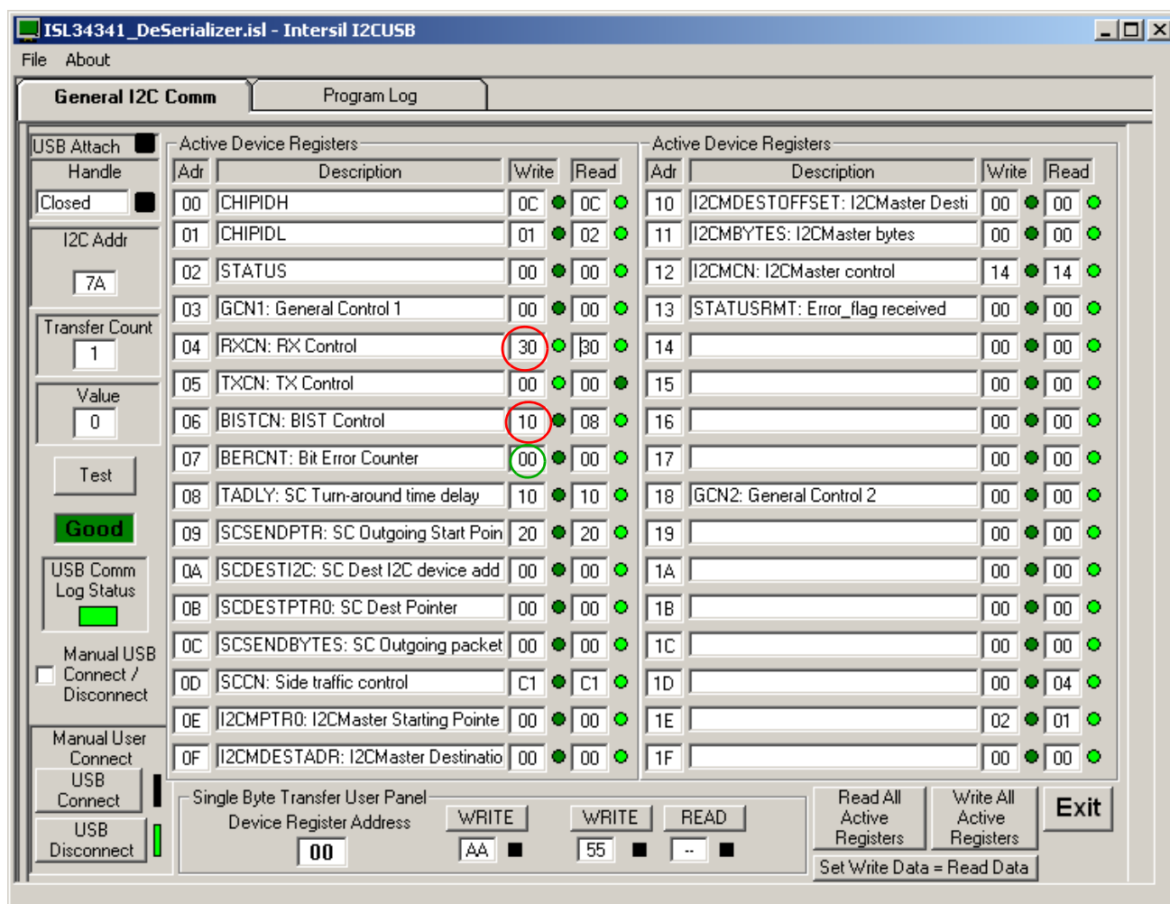
FIGURE 9. DESERIALIZER CONFIGURATION
