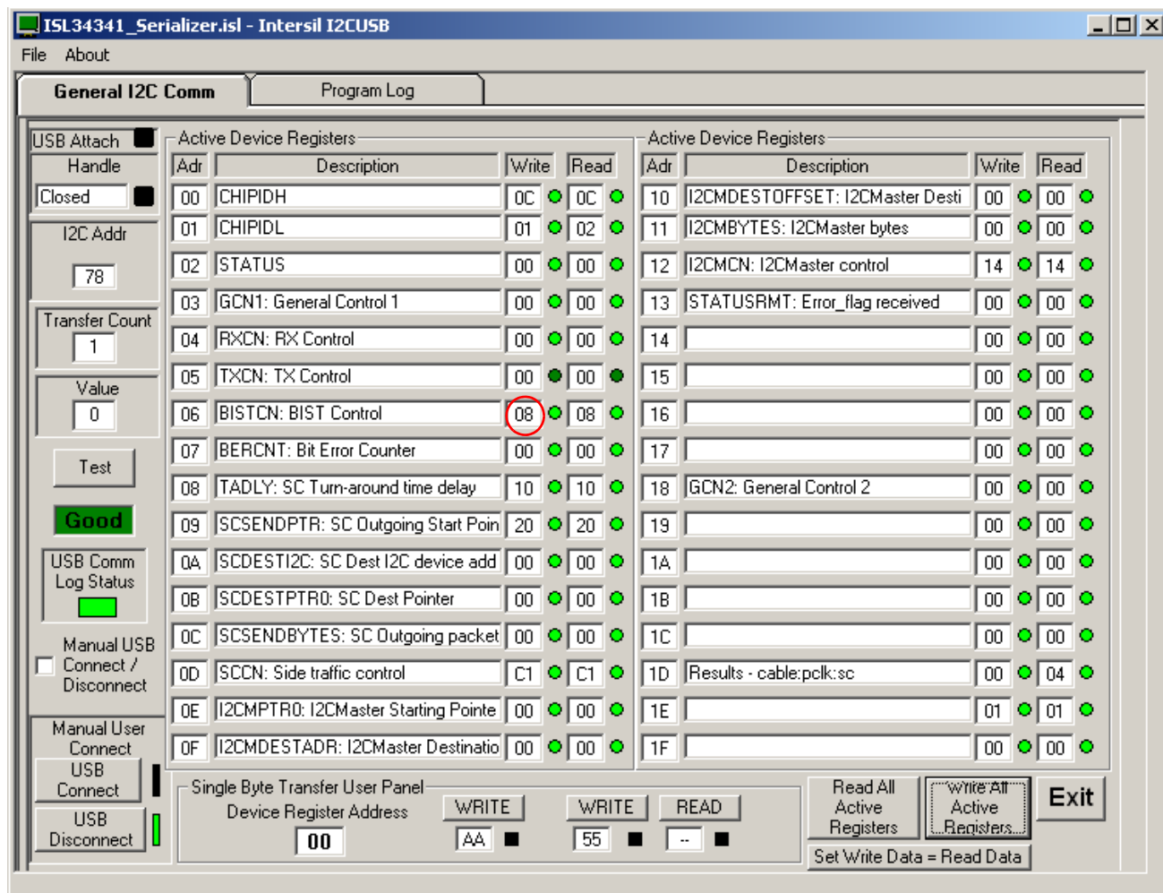
FIGURE 8. SERIALIZER CONFIGURATION
