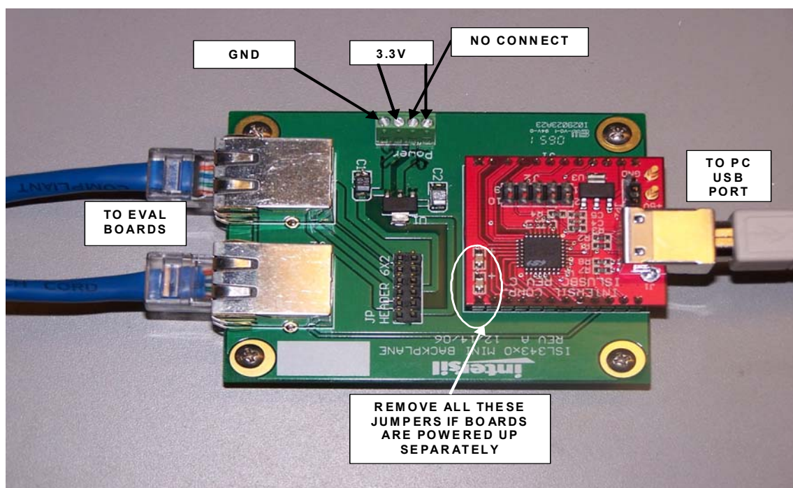
FIGURE 3. INTERFACE BOARD
