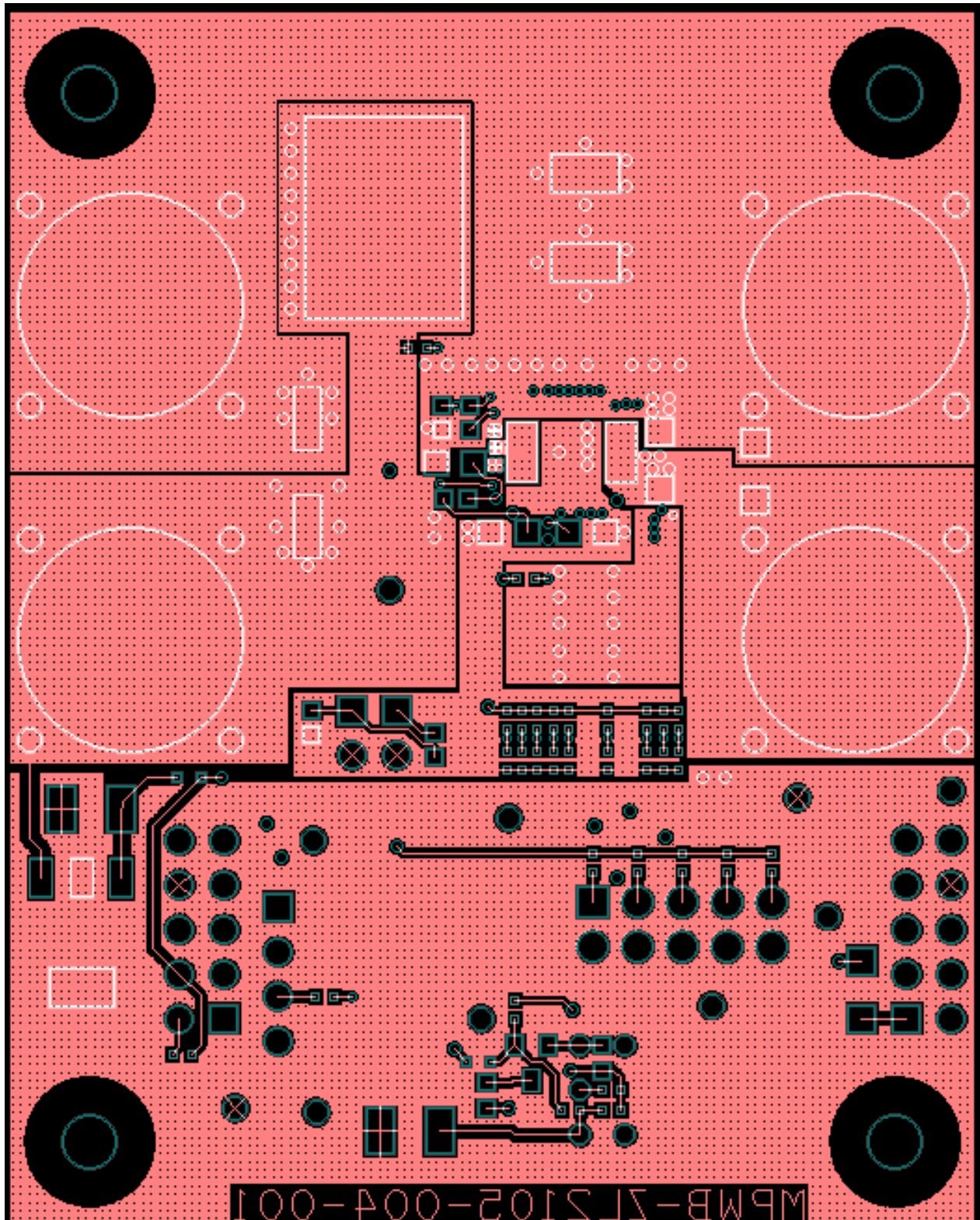
Figure 9. PCB – Bottom Layer (Viewed from Top)
