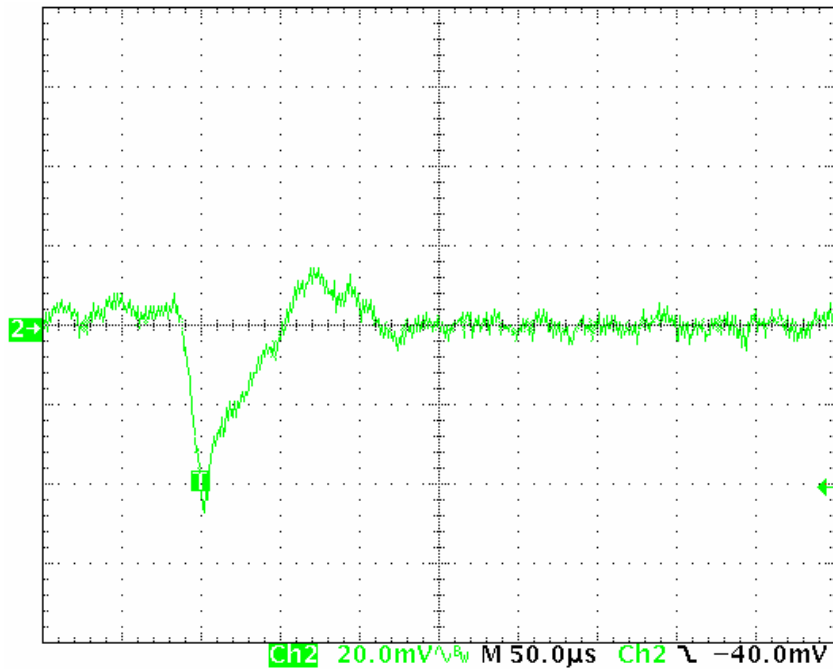
Figure 12. Dynamic Response (1 - 2A load step, di/dt=1A/\mu s )
