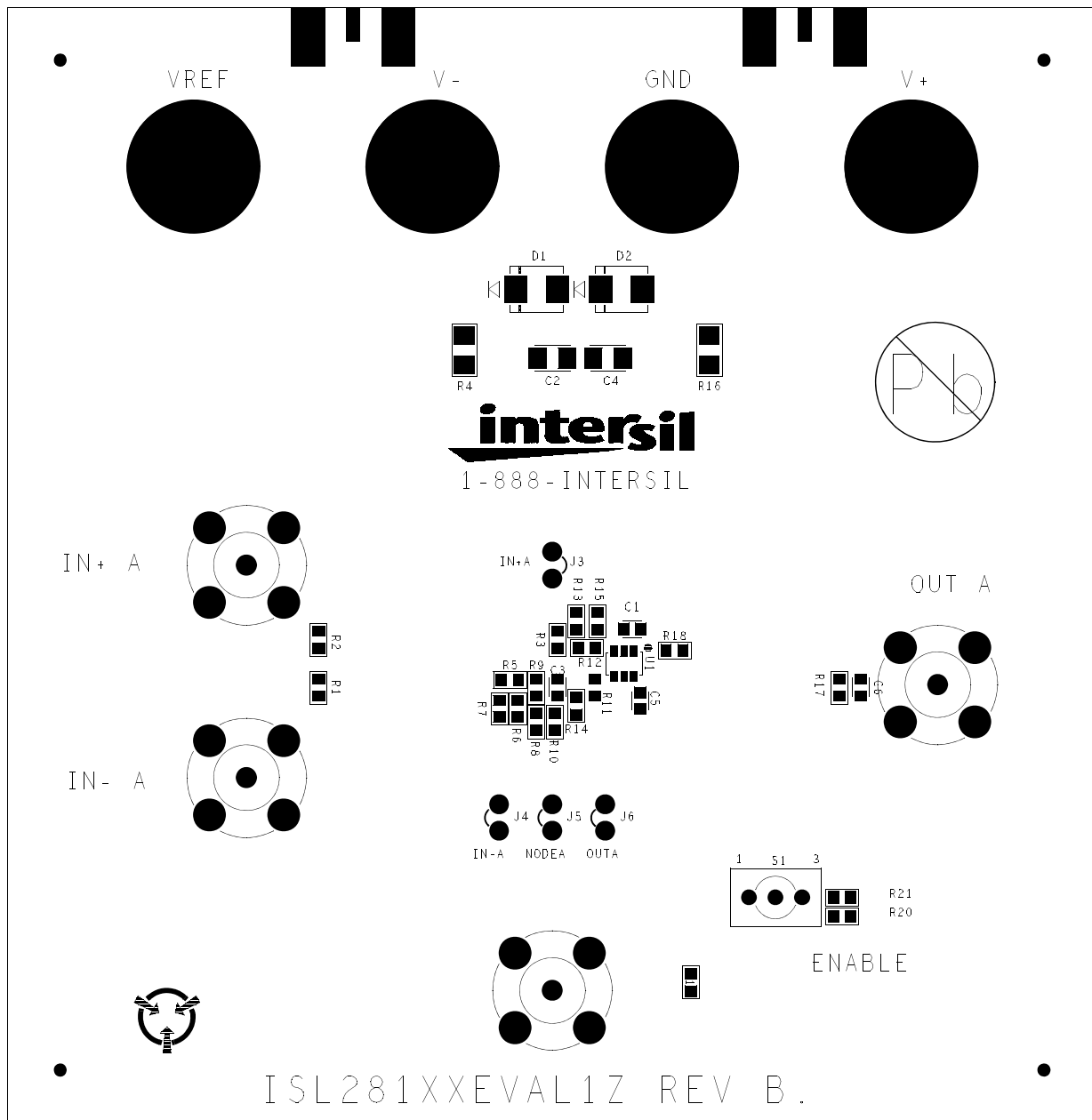
FIGURE 5. TOP VIEW
