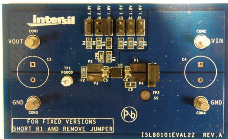
FIGURE 1. ISL80101EVAL2Z
