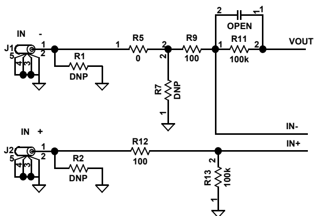
FIGURE 3. INPUT STAGE
