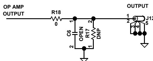
FIGURE 4. OUTPUT STAGE
