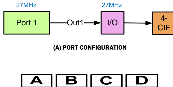
FIGURE 29. PORT SETTING EXAMPLE 5 : 4-CIF
