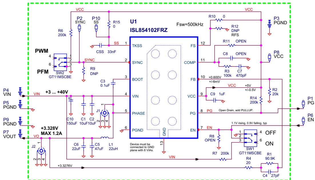
FIGURE 9. ISL854102EVAL1Z SCHEMATIC
