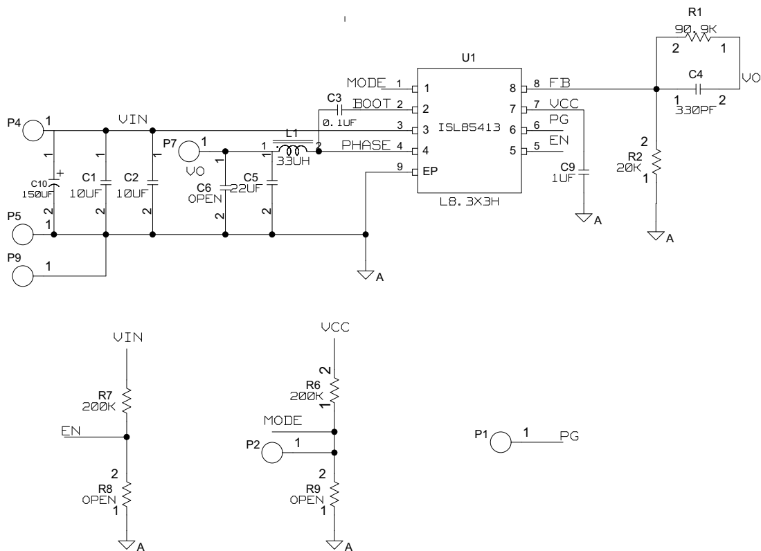
FIGURE 2. ISL85413DEM01Z AND ISL85412DEM01Z SCHEMATIC
