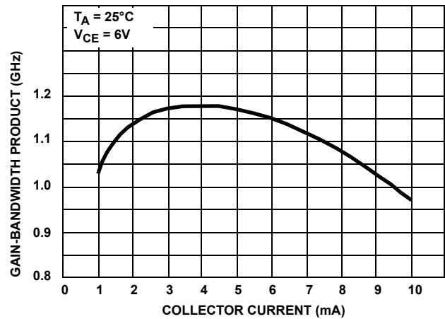
FIGURE 6. GAIN-BANDWIDTH PRODUCT vs COLLECTOR CURRENT
