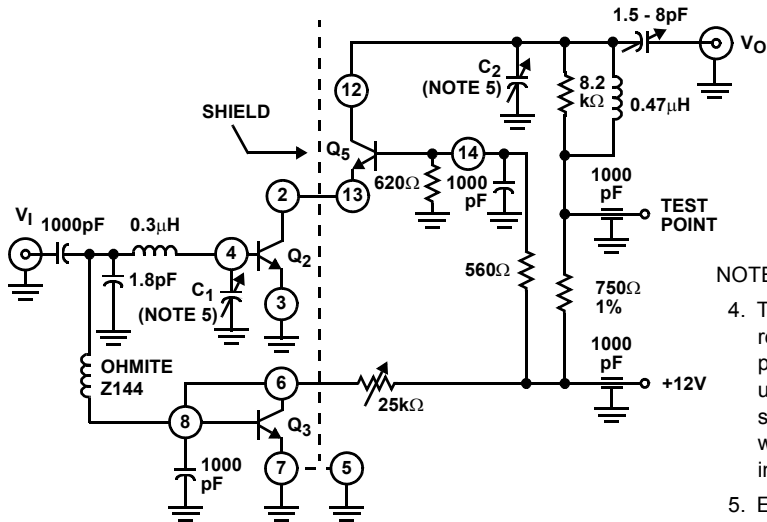
FIGURE 2. 100MHz POWER-GAIN AND NOISE-FIGURE TEST CIRCUIT
