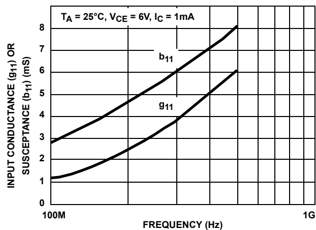
FIGURE 12. INPUT ADMITTANCE ( Y_{11} ) vs FREQUENCY
