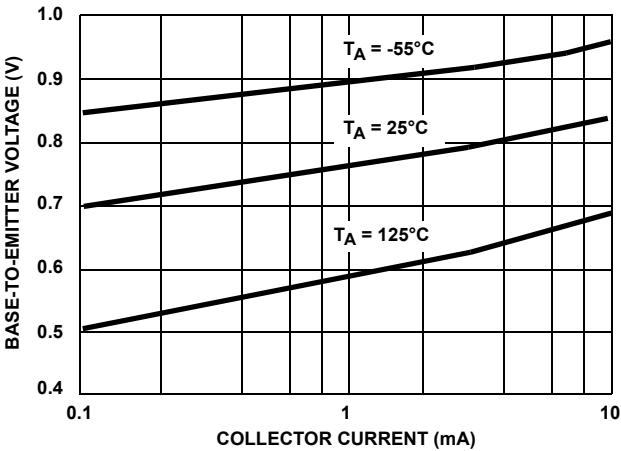
FIGURE 7. BASE-TO-EMITTER VOLTAGE vs COLLECTOR CURRENT
