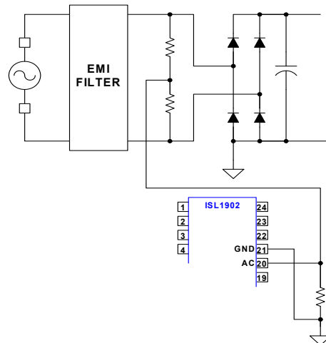
FIGURE 17. AC DETECTION
