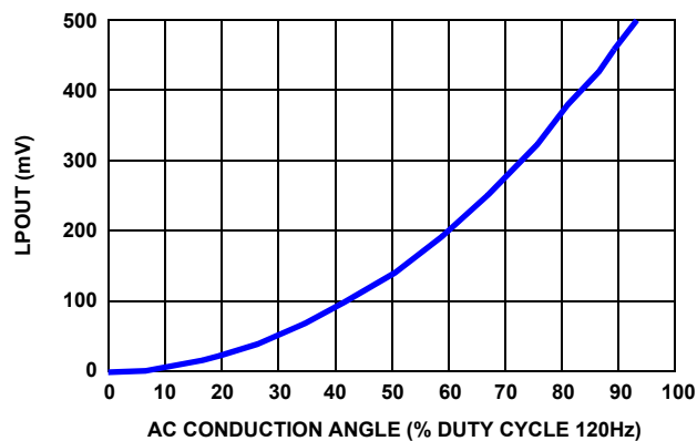
FIGURE 4. LPOUT vs AC SIGNAL DUTY CYCLE
