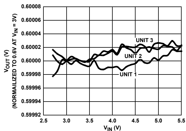
FIGURE 4. LINE REGULATION
