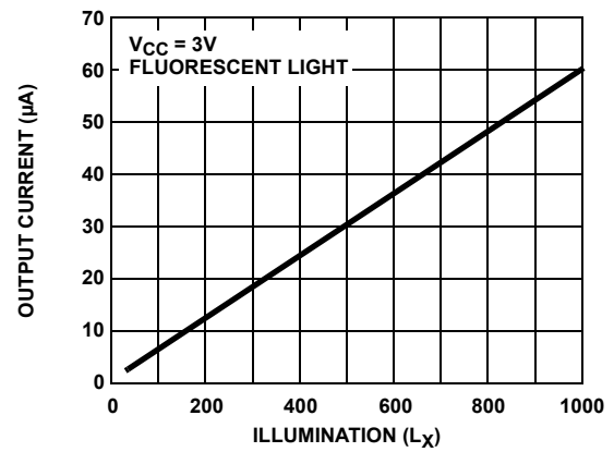
FIGURE 4. SENSITIVITY
