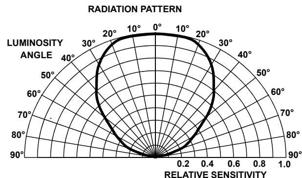
FIGURE 7. RADIATION PATTERN
