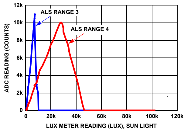
FIGURE 17. SATURATION CHARACTERISTICS
