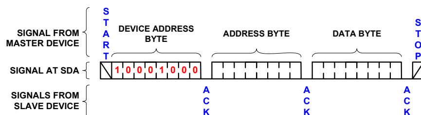
FIGURE 11. BYTE WRITE SEQUENCE
