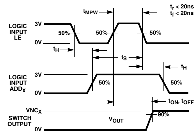
FIGURE 3. BREAK-BEFORE-MAKE TIME
