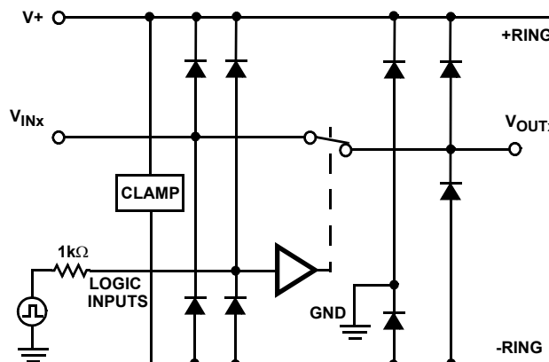
FIGURE 8. OVERVOLTAGE PROTECTION
