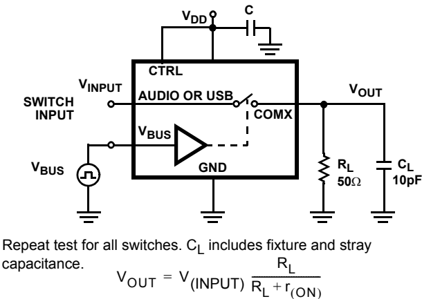
FIGURE 1B. TEST CIRCUIT
